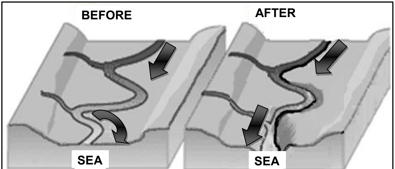
FIGURE 1.6: RIVER REJUVENATION
