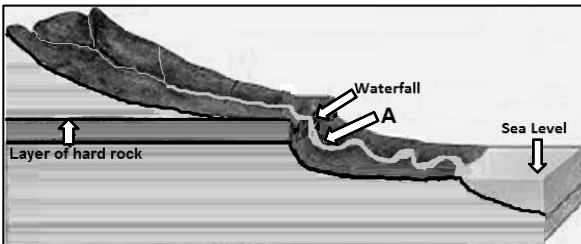
FIGURE 2.6: RIVER PROFILE
