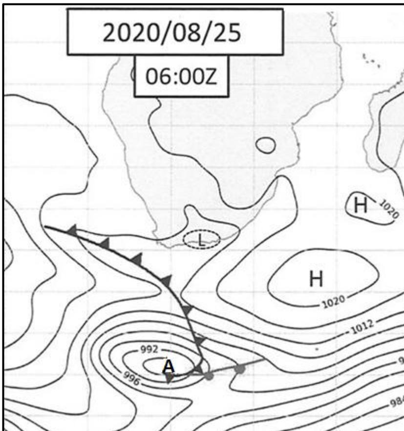
FIGURE 1.3: MID-LATITUDE CYCLONE
